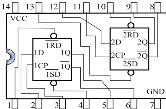
74xx74
