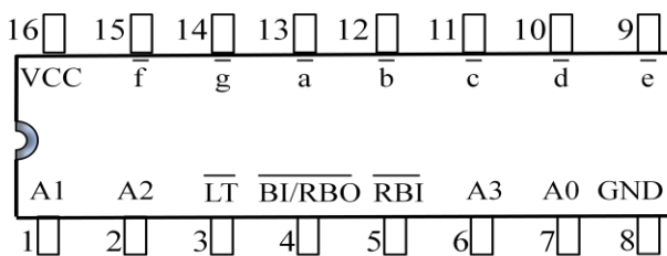
74xx47
